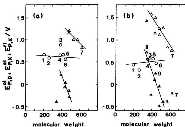
Fig. 6. Plots of E_p^1 of D, and E_p^1,X and E_p^2,X of X^- vs. the molecular weight. (a), in THF; (b), in BN. (O), E_p^1,D ; ( \Delta ), E_p^1,X ; ( \blacktriangle ), E_p^2,X . 1: TTF, 2: TMTTF, 3: TMT-TTF, 4: BEDT-TTF, 5: BTDT-TTF, 6: TMTSF, 7: \text{I}_3^- , 8: \text{Cl}_3^- , 9: \text{BrCl}_2^- .
